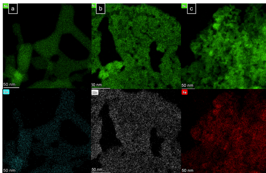
Fig. 3 STEM-EDS maps of a) 10% Co, b) 10% Mn, and c) 10% Fe NiO(111) showing the distribution of the dopants across the NiO sheets.
