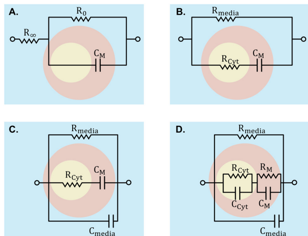
Fig. 7 ECMs employed to interpret signals into cell properties. A) Cole model, wherein R_{\text{inf}} and R_0 denote high and low-frequency resistance, respectively. B) Fricke model. C) and D) are extensions of the Fricke model integrating supplementary elements for increased precision. In these models, while R and C signify resistance and capacitance, the M subscript designates membrane properties, \text{Cyt} represents cytoplasm properties, and 'media' denotes properties of the surrounding medium.
