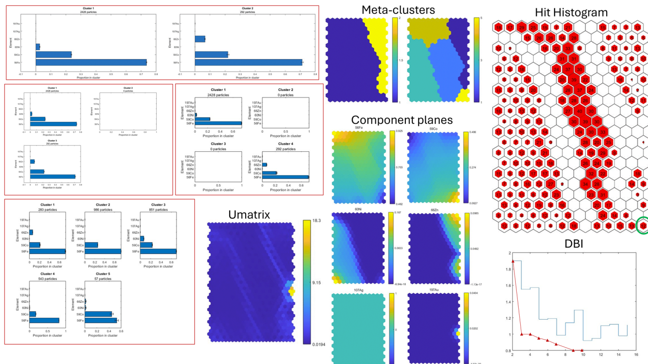
Fig. 5 Particle differentiation SOM outputs, DBI analysis results, and elemental composition of FeCoNi/Zn ENP meta-clusters based on 9 MCS particle detection som.
