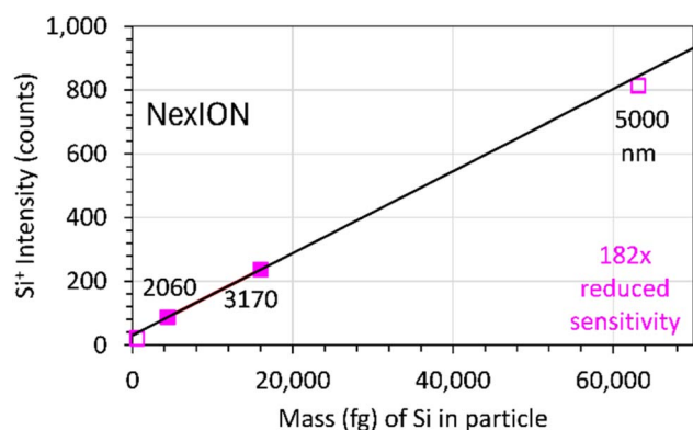
Fig. 7 ^{28}\text{Si}^+ signal in counts produced by engineered \text{SiO}_2 particles measured by spICP-QMS using 182x reduced sensitivity. The nominal particle diameter is shown next to each point. Filled symbols indicate particles used to calculate the linear regression line while open symbols indicate particles not used to calculate the linear regression line.
