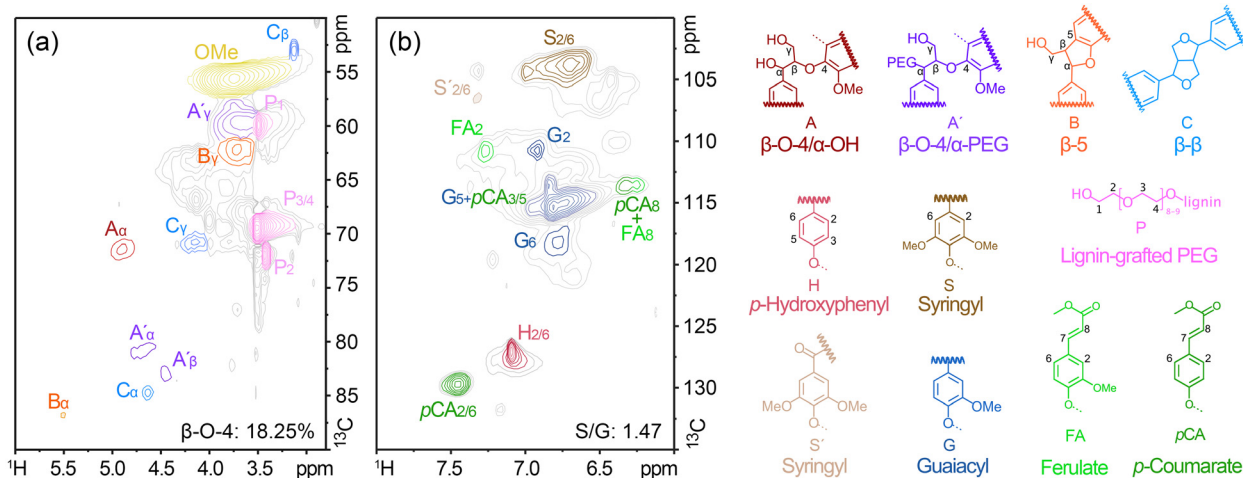
Fig. 5 2D HSQC NMR spectra of PEG-g-lignin obtained from the biphasic fractionation process. (a) Side-chain region ( \delta C/\delta H 90–50/6.0–2.75) and (b) aromatic region ( \delta C/\delta H 135–100/8.0–6.0).
