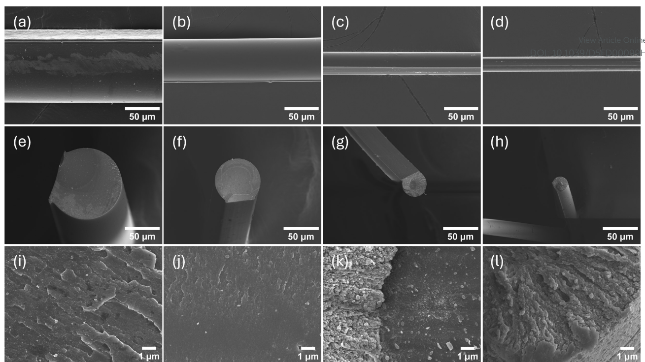
Figure 2. SEM images of the fibre lengths of 25 G as-spun lignin-PVA fibres (a), and hot-drawn fibres at 180 °C to DR 2.5 (b), DR 8 (c), and DR 20 (d). The respective cross-sections are seen at the same magnification (e-h) and at higher magnification (i-l).
