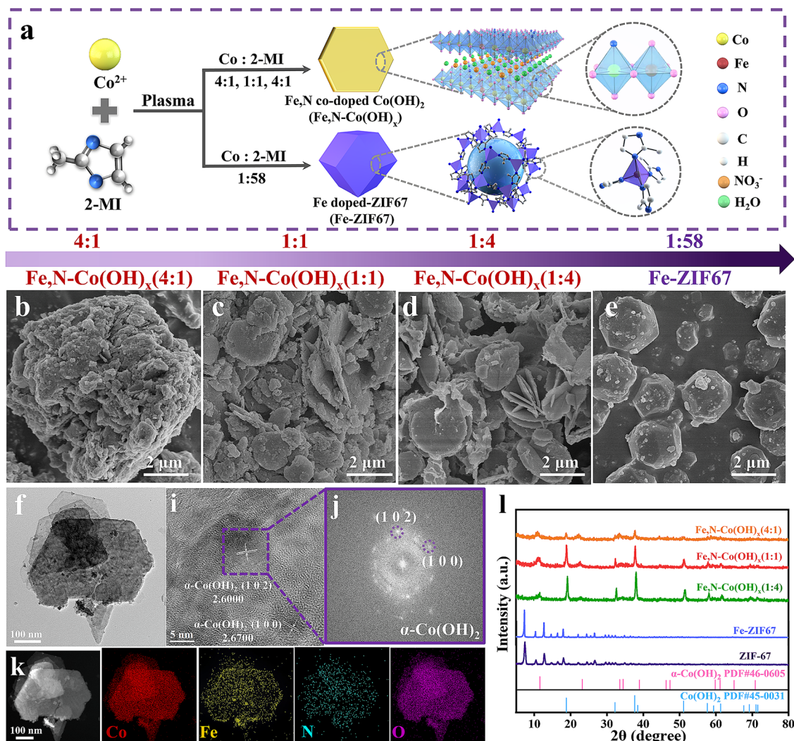
Fig. 1 Preparation process and morphology of electrocatalysts. (a) Schematic of the synthesis of \text{Fe,N co-doped Co(OH)}_2 (i.e., \text{Fe,N-Co(OH)}_x ) and \text{Fe-doped ZIF67} (i.e., \text{Fe-ZIF67} ) induced by plasma in water. (b)–(e) SEM images of (b) \text{Fe,N-Co(OH)}_x (4:1), (c) \text{Fe,N-Co(OH)}_x (1:1), (d) \text{Fe,N-Co(OH)}_x (1:4), and (e) \text{Fe-ZIF67} . (f)–(k) Morphology and elemental distribution of \text{Fe,N-Co(OH)}_x (1:1): (f) TEM images, (g) HAADF-STEM images, (h) corresponding FFT pattern, and (i)–(k) EDS mapping images. (l) XRD patterns of \text{Fe,N-Co(OH)}_x (4:1) (orange line), \text{Fe,N-Co(OH)}_x (1:1) (red line), \text{Fe,N-Co(OH)}_x (1:4) (green line), and \text{Fe-ZIF67} (purple line).
