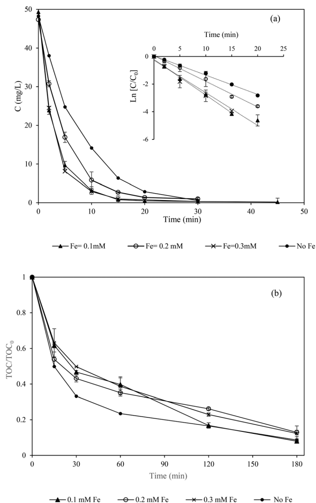
Fig. 4 Effect of iron catalyst Fe^{2+} concentration on MCZ degradation (a) and mineralization (b) during electro-Fenton treatment at a constant current intensity of 150 mA, Na_2SO_4 = 50 mM and pH = 3.
