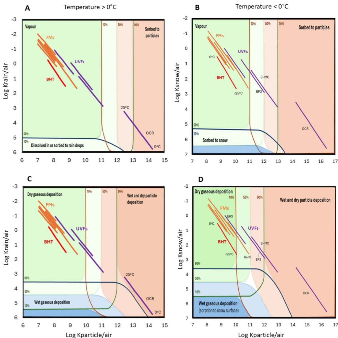
Fig. 4 Equilibrium phase distribution of the 12 PCPs in a warm (temperature range 0 to 25 °C) (A) and a cold (temperature range 0 to −25 °C) (B), and the dominant atmospheric deposition processes at temperatures above (C) and below (D) 0 °C. They are a function of the particle-air, rain-air, and snow-air distribution ratios. The green areas represent dominant gas phase distribution (A and B), and dry gaseous deposition (C and D). Red areas designate particle sorption (A and B), and wet and dry deposition (C and D). Finally, blue areas show liquid water (A) or snow (B) distribution, and wet gaseous deposition (C and D).
