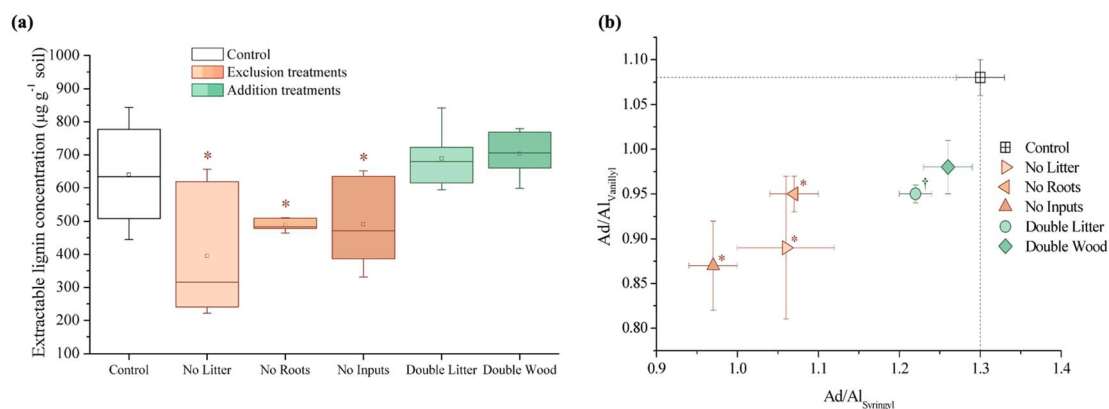
Fig. 3 Concentration ( \mu\text{g g}^{-1} soil) indices of compounds isolated through the cupric oxidation of forest soil samples after 20 years of detrital manipulation experiments at the Sikfőkút Experimental Forest: (a) total extractable lignin-derived compounds and (b) acid-to-aldehyde (Ad/Al) ratios for the vanillyl vs. syringyl monomers. An asterisk (*) denotes treatments significantly different ( p \leq 0.05 ) from the control. A dagger (†) denotes when only the vanillyl Ad/Al ratio was significantly different ( p \leq 0.05 ) from the control.
