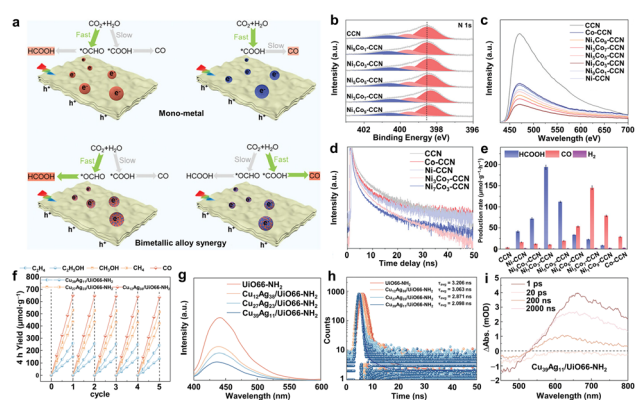
Fig. 5 (a) Schematic diagram of the reaction mechanism of photoreduction of \text{CO}_2 by the \text{Ni}_x\text{Co}_y -CCN catalyst. (b) XPS spectra of N 1s, (c) PL spectra and (d) time-resolved transient PL decay spectra for \text{Ni}_x\text{Co}_y -CCN. (e) Product evolution rates of \text{Ni}_x\text{Co}_y -CCN. Reproduced with permission from ref. 50. Copyright 2024, Wiley-VCH. (f) The cycling test over \text{CuAg}_{50-x}/\text{UiO66-NH}_2 . (g) PL spectra; (h) time-resolved transient PL decay spectra and (i) Fs-TA spectra of \text{CuAg}_{50-x}/\text{UiO66-NH}_2 . Reproduced with permission from ref. 51. Copyright 2024, Royal Society of Chemistry.
