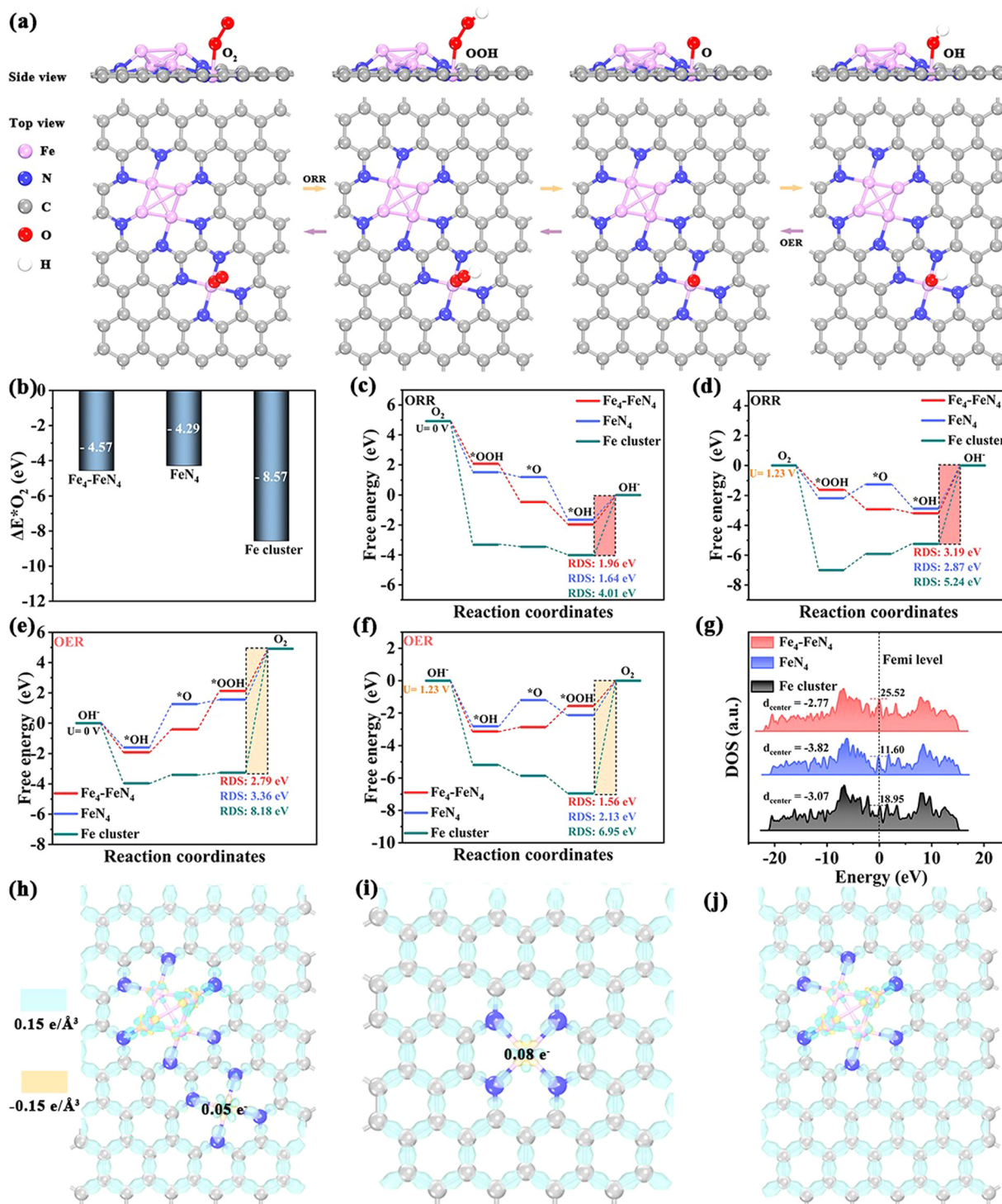
Fig. 4 DFT calculations. (a) Side and top views of the oxygen-containing intermediates adsorbed on Fe 4 -FeN 4 models at the Fe site of FeN 4 . (b) O 2 adsorption energy values on the Fe sites of Fe 4 -FeN 4 , FeN 4 and Fe cluster models. Free energy diagrams of intermediate species in the (c) and (d) ORR and (e) and (f) OER processes for Fe 4 -FeN 4 , FeN 4 and Fe cluster models at U = 0 V and U = 1.23 V. (g) DOS of Fe 4 -FeN 4 , FeN 4 , and Fe cluster models. Differential charge density of (h) Fe 4 -FeN 4 , (i) FeN 4 and (j) Fe cluster models.
