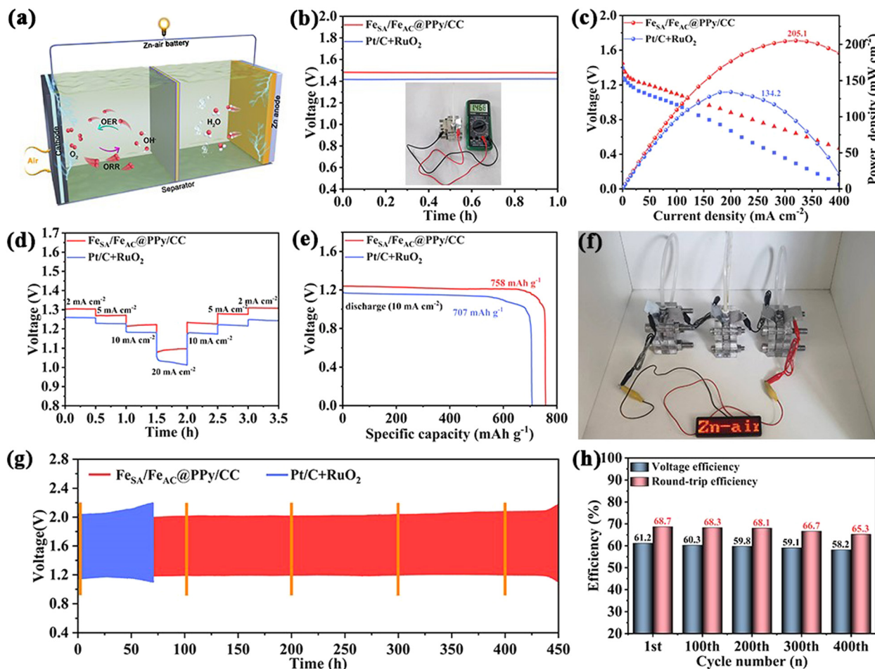
Fig. 5 Aqueous rechargeable ZAB performances. (a) Scheme of aqueous ZAB. (b) Open-circuit voltages. (c) Discharging curves and the corresponding power density plots. (d) Discharging curves at 2–20 \text{mA cm}^{-2} . (e) Specific discharging capacities at 10 \text{mA cm}^{-2} for \text{Fe}_{\text{SA}}/\text{Fe}_{\text{AC}}@\text{PPy}/\text{CC} and \text{Pt}/\text{C}+\text{RuO}_2 -based ZABs. (f) Photo of three \text{Fe}_{\text{SA}}/\text{Fe}_{\text{AC}}@\text{PPy}/\text{CC} -based ZABs driving a 4 V LED viewing screen. (g) Long-term galvanostatic charging–discharging plots of \text{Fe}_{\text{SA}}/\text{Fe}_{\text{AC}}@\text{PPy}/\text{CC} and \text{Pt}/\text{C}+\text{RuO}_2 -based ZAB at a current density of 10 \text{mA cm}^{-2} . (h) Voltage efficiency and round-trip efficiency of \text{Fe}_{\text{SA}}/\text{Fe}_{\text{AC}}@\text{PPy}/\text{CC} at 1, 100, 200, 300, and 400 cycles of (g).
