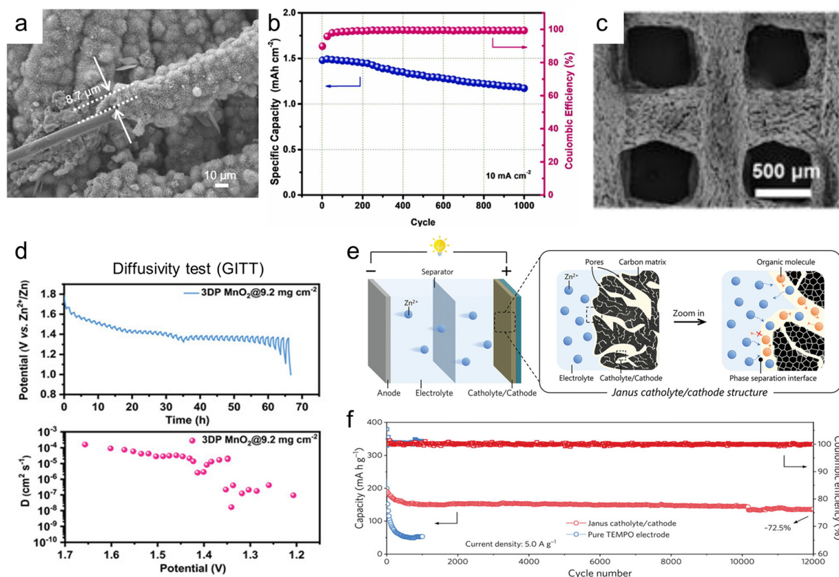
Fig. 13 Electrode-level energy enhancement via architecture strategies for thick cathode design. (a) SEM images of KMO NWs. (b) Cycling performance of the Zn||KMO NWs battery at a current density of 10 \text{ mA cm}^{-2} . Reproduced with permission from ref. 247. Copyright 2024, Elsevier. (c) Top-view SEM images of 3DP CMs. (d) GITT profiles and corresponding D values in 3DP \text{MnO}_2 electrode at \text{MnO}_2 mass loading of 9.2 \text{ mg cm}^{-2} during discharging process. Reproduced with permission from ref. 248. Copyright 2023, Wiley-VCH. (e) Schematic illustration of the working mechanism for rechargeable Zn||Janus catholyte/cathode cell. (f) Long-term cycling performances and coulombic efficiencies at current densities of 5.0 \text{ A g}^{-1} of Janus catholyte/cathode and pure TEMPO electrode. Reproduced with permission from ref. 249. Copyright 2024, Wiley-VCH.
