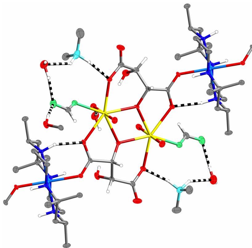
Fig. 1 A fragment within the structure of [(\text{CH}_3)_2\text{NH}_2]_2[(\text{UO}_2)_2(\text{HTRT})_2(\text{HCO}_2)_2\text{Ni}(\text{R},\text{S-Me}_6\text{cyclam})]\cdot 2\text{H}_2\text{O} ( \text{HTRT}^- = hydrogentartrate) 92 showing the part of the intricate network of hydrogen bonds (dashed lines) that link dimethylammonium counterions, water and coordinated formate. For clarity, CH atoms are shown only on the coordinated tartrate and formate units, with formate oxygen shown in green and dimethylammonium nitrogen in pale blue. Otherwise U = yellow, Ni = sky blue, N = dark blue, and O = red, H = white spheres with an arbitrary radius of 0.1 Å, with other atom displacement ellipsoids shown at the 80% level (figure prepared using CrystalMaker 11.5 from CrystalMaker Software Ltd).
