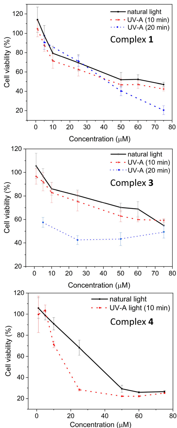
Fig. 7 Photocytotoxicity of the metal complexes ( 1 , 3 and 4 ) in the HeLa tumor cell line. Cells were treated with different concentrations of the metal complexes (1–75 μM), followed by 365 nm photo-irradiation and incubation for 72 h at 37 °C. The natural light and 365 nm photo-irradiated cells are shown by a solid line and dotted line, respectively. Data were averaged, and the standard deviation was calculated with the multiple determinations of each substance and concentration. Depicted are the mean values and standard deviation from n = 6 experiments.
