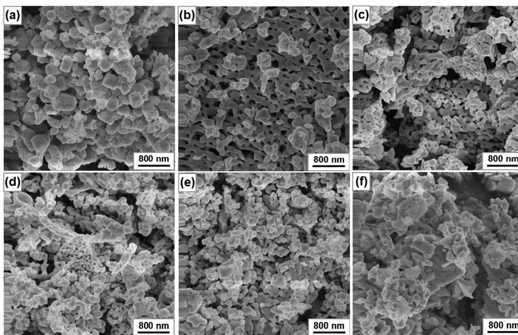
Fig. 2 SEM images of the as-received Ta 2 O 5 (a) and 0.35-O 2 (b), 0.25-O 2 (c), 0.15-O 2 (d), 0.05-O 2 (e), and 0-O 2 (f) samples synthesized under oxygen partial pressures ( p_{O_2} ) of 0.35, 0.25, 0.15, 0.05, and 0 L h -1 , respectively.
