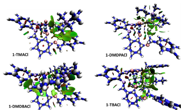
Fig. 14 Isosurface maps of \text{IRI} = 1 for all structures computed from crystallographic coordinates. Blue regions are associated with covalent or coordination bonds, green regions with dispersive interactions and red regions with repulsive interactions. Color chart: H = white, C = grey, N = violet, O = red, Cl = lime, U = light blue.
