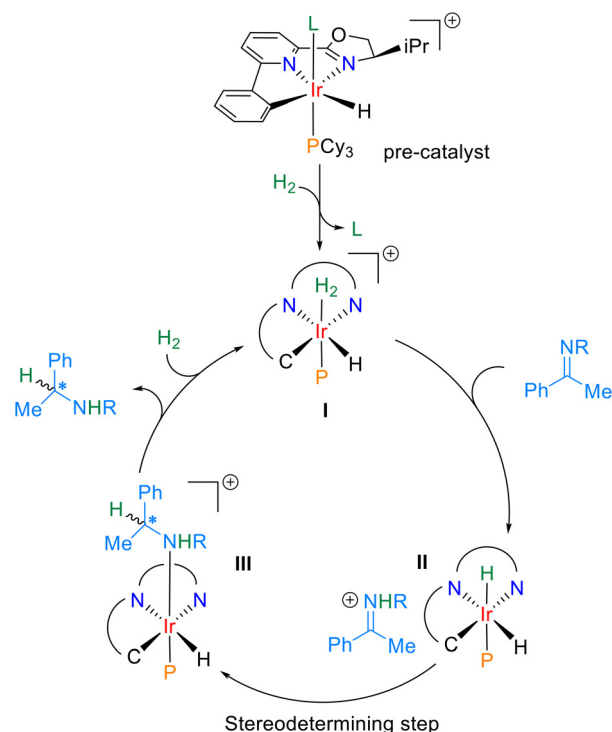
Fig. 4 Hydrogenation mechanism with Ir(III) octahedral catalysts.
