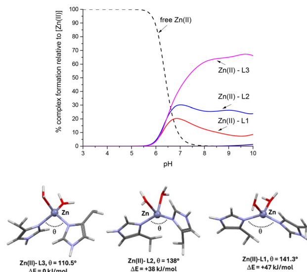
Fig. 8 Top: competition plot between L1 (KSHFELPHYPGL), L2 (kshfelphypgl) and L3 (lgpyhplefhsK) with Zn(II) ions describing complex formation at different pH values in a hypothetical situation, in which equimolar amounts of the all reagents are mixed. Conditions: T = 298\text{ K} , [\text{Zn(II)}] = [\text{L1}] = [\text{L2}] = [\text{L3}] = 0.001\text{ M} . Bottom: calculated coordination environment of the Zn(II) ion in the three systems at pH range of 5.5–7.0 (for L3 both [\text{ZnH}_3\text{L}_3]^{2+} and [\text{ZnH}_2\text{L}_3]^+ complex species and for L2 and L1 in [\text{ZnH}_2\text{L}]^+ complex species). \Delta E indicates the relative energy of the systems with Zn(II)–L3 being the most stable.
