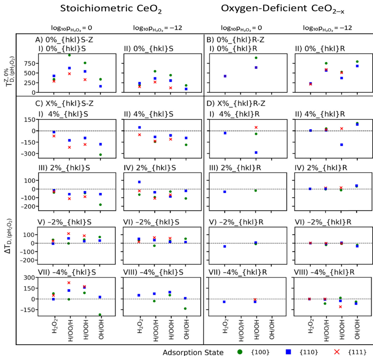
Fig. 3 Desorption temperature of molecularly and dissociatively adsorbed hydrogen peroxide on stoichiometric and oxygen-deficient \text{CeO}_2 . T_{\text{D}}^{\text{N.O.}}(p_{\text{H}_2\text{O}_2}) of adsorbed hydrogen peroxide species on unstrained stoichiometric (A) and oxygen-deficient (B) \text{CeO}_2 surfaces. \Delta T_{\text{D}}(p_{\text{H}_2\text{O}_2}) of adsorbed hydrogen peroxide species on strained stoichiometric (C) and oxygen-deficient (D) \text{CeO}_2 surfaces.
