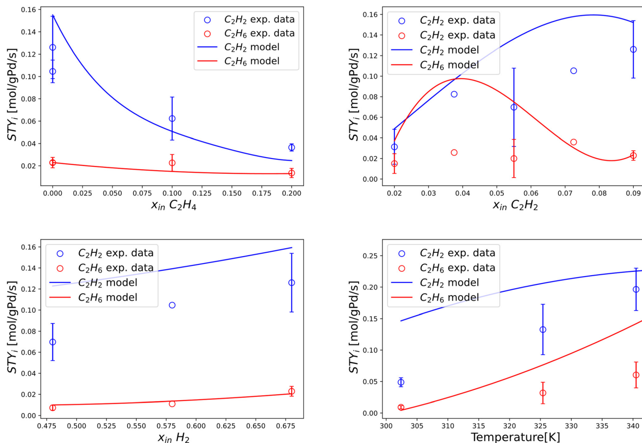
Fig. 10 Experimentally measured and modelled space-time yields of C_2H_2 consumption and C_2H_6 production ( STY_{C_2H_2} [mol g_{Pd}^{-1} s ^{-1} ] and STY_{C_2H_6} [mol g_{Pd}^{-1} s ^{-1} ]) plotted against single manipulated operating variables. Top left) Trends vs. inlet molar fraction of C_2H_4 obtained at 293 K, i.e. 20 °C. Top right) Trends vs. inlet molar fraction of C_2H_2 obtained at 293 K, i.e. 20 °C. Bottom left) Trends vs. inlet molar fraction of H_2 obtained at 293 K, i.e. 20 °C. Bottom right) Trends vs. isothermal reactor temperature. Includes experimental data from this work and model simulation results by this work. The standard deviation of experimental measurements is reported through error bars for points whose reproducibility has been verified through at least two repeated experiments.
