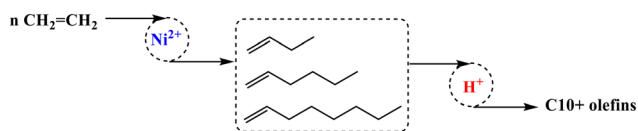
Scheme 15 Main reaction pathways of ethylene oligomerization into C 10+ olefins by catalytic cascade reactions.
