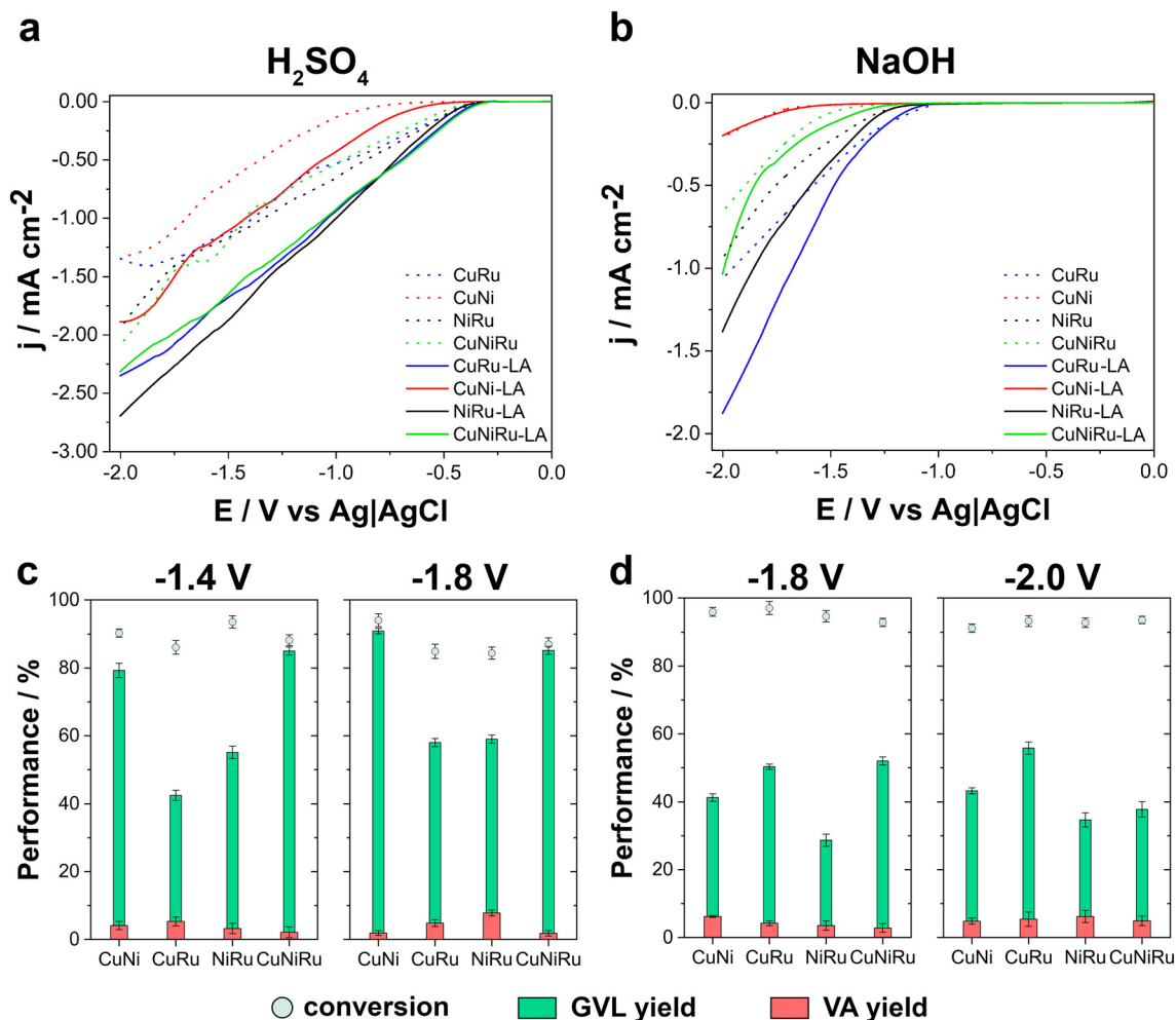
Fig. 5 Linear sweep voltammograms (LSV) recorded within a potential range of 0.0 V to -2.0 V vs. Ag|AgCl|Cl - at a scan rate of 50 \text{ mV s}^{-1} , in the absence (dashed line) and presence (solid line) of 0.5 \text{ M} of LA, using CuRu, CuNi, NiRu, and CuNiRu electrodes in (a) acidic and (b) basic media. Conversion percentages and product selectivity toward GVL and VA in (c) acidic and (d) basic media. All experiments were performed in triplicate, with values reported as the mean \pm standard deviation.
