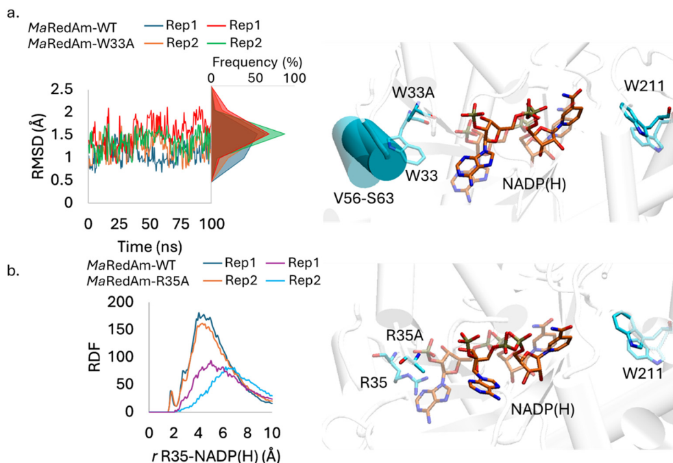
Fig. 2 RMSD of V56-S63 \alpha -helix obtained from molecular dynamics (MD) simulations of MaRedAm-WT and MaRedAm-W33A systems (a). RDFs of R35-NADP(H) pair calculated from MD simulations of MaRedAm-WT and MaRedAm-R35A systems (b). For clarity, hydrogens were omitted, and only relevant species were reported. In the figures, atoms in transparent-background representation are for the wild-type enzyme.
