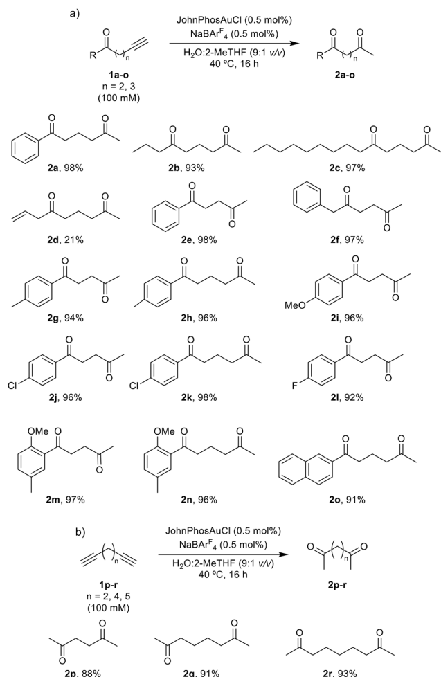
Scheme 2 a) Synthesis of \gamma - and \delta -diketones 2a–o through the Au(I)-catalyzed alkyne hydration reaction. b) Synthesis of aliphatic diketones 2p–r starting from 1,6-diynes.
