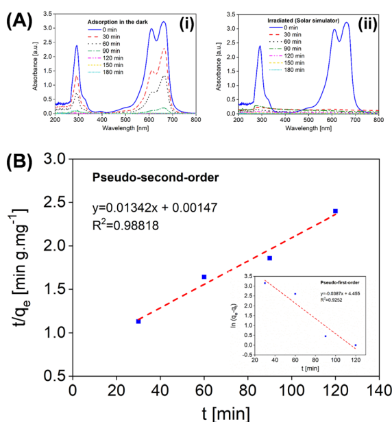
Fig. 4 (A) Kinetics of MB adsorption (i) in the dark and (ii) under solar irradiation (initial dye concentration 25 mg L -1 , catalyst amount 0.5 g L -1 , volume of solution 40 mL). (B) Pseudo-second-order kinetic plot (inset is pseudo-first-order kinetic plot).
