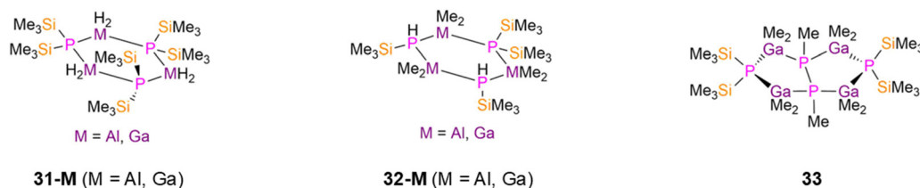
Fig. 8 Polynuclear 13 P'' complexes [\text{M}(\text{H})_2(\mu\text{-P}'')]_3 ( 31-M : M = \text{Al, Ga} ), \{[\text{M}(\text{Me})_2(\mu\text{-P}'')]\text{HP}(\text{SiMe}_3)_2\}_2 ( 32-M : M = \text{Al, Ga} ), \{[\text{Ga}(\text{Me})_2(\mu\text{-P}'')]_2(\mu\text{-P}(\text{Me}))_2\} ( 33 ).
