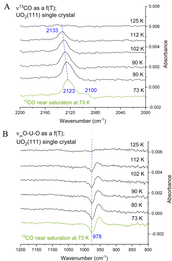
Fig. 5 (A) Difference IRRAS spectra for \nu^{13}\text{CO} at near saturation (0.2 L exposure) on \text{UO}_2(111) single crystal at 73 K followed by flashing the crystal at a rate of 0.1\text{--}0.2\text{ K s}^{-1} to the indicated temperature then cooled to 73 K for further collection. (B) The low frequency region ( 1200\text{--}800\text{ cm}^{-1} ), note the absence of change in the wavenumber with temperature.
