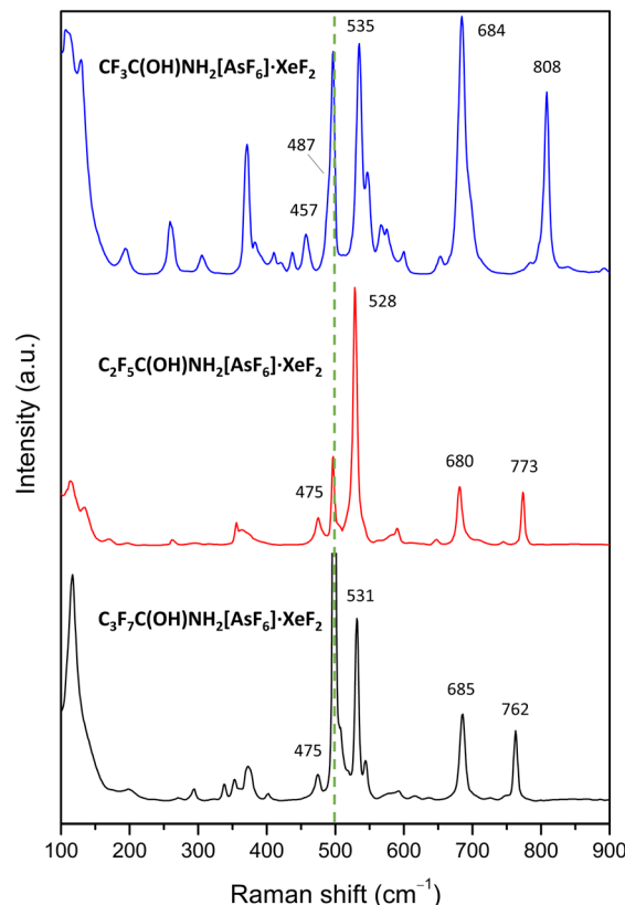
Fig. 8 Raman spectra of \text{XeF}_2 salt cocrystals with protonated amides recorded at low temperatures ( -90^\circ\text{C} ). The green dashed line is placed at the position of free \text{XeF}_2 (497 \text{cm}^{-1} ) 41 which was observed as an impurity in the reactions.
