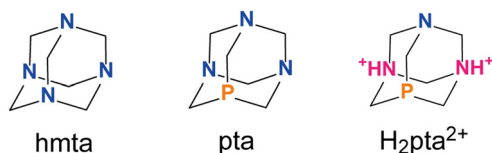
Fig. 1 Molecular structures of hmta, pta and H_2pta^{2+} .
