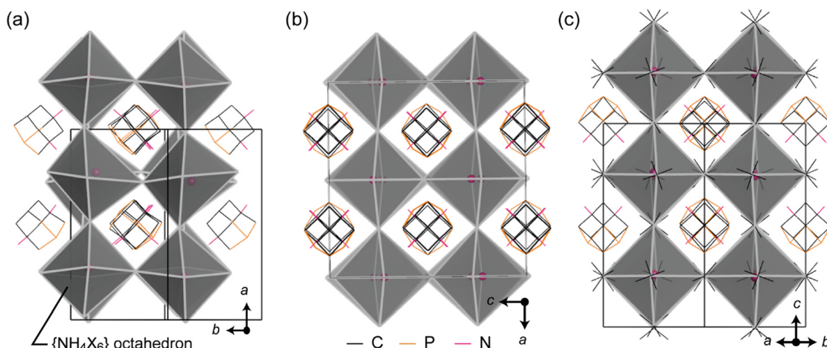
Fig. 2 Crystal structures of (a) p-Br , (b) p-I and (c) p-BF 4 . H atoms on C atoms were omitted except for the N^+-H bond shown by the red line. The octahedron represents the \{NH_4X_6\} structural unit where the black lines in (c) represent B–F bonds.
