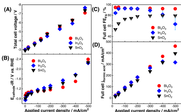
Fig. 3 (A) Total full-cell cell voltages ( E_{\text{cell}} ) and (B) GDE half-cell iR -corrected cathode potentials ( E_{\text{cathode}}-iR ) versus total applied current density. Comparison of (C) \text{FE}_{\text{FA}} and (D) FA partial current density versus total applied current density in the full-cell device for \text{Bi}_2\text{O}_3 , \text{In}_2\text{O}_3 , and \text{SnO}_2 .
