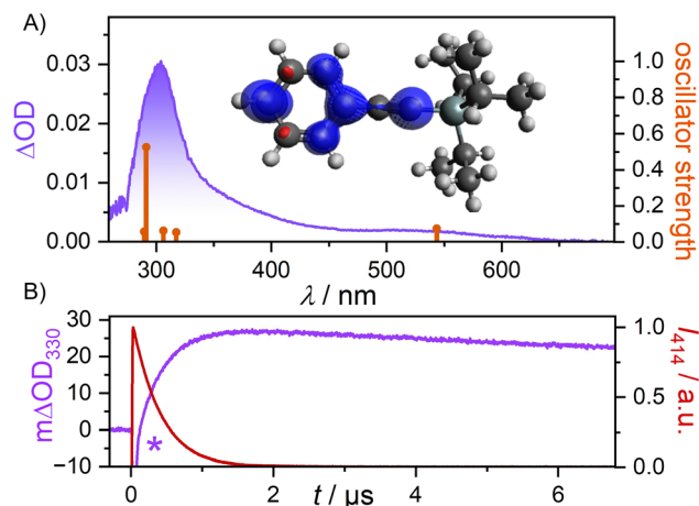
Fig. 3 TA measurements of Ir and TIPS-Bz in Ar-saturated benzene with 355 nm laser pulses (A) TA spectrum of Ir (6.25 \mu M) and 1 mM TIPS-Bz recorded 4 \mu s after excitation shown together with the oscillator strength calculated by TD-DFT (B3LYP/6-311+G(d,p) level of theory). (B) Kinetic measurements of Ir (25 \mu M) emission and transient absorption of TIPS-Bz (2 mM).
