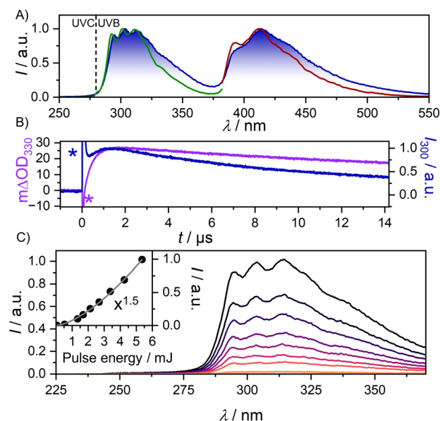
Fig. 4 Mechanistic investigations of 25 \mu M Ir and 2 mM TIPS-Bz in Ar-saturated benzene. (A) Time-gated emission spectrum after 355 nm laser pulse excitation (blue, 4–204 \mu s) and after 280 nm excitation (green and red, normalized to the maximum in the UV and visible region). (B) Kinetic traces of the ^1\text{TIPS-Bz}^* emission and transient absorption of ^3\text{TIPS-Bz}^* . (C) Excitation-intensity dependent delayed emission spectra. Inset: Emission maximum plotted against laser pulse intensity with a pulse duration of \sim 5 ns. See text for details.
