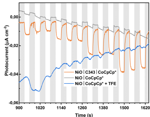
Fig. 4 Chopped light amperometry experiment with 10 mM of 1, showing generated photocurrent upon illumination (from 900 seconds onwards). Control experiments in grey and blue. Cell was illuminated for periods of 30 seconds (indicated by white bars) by a white LED with 100\text{ mW cm}^{-2} intensity.
