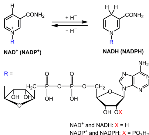
Fig. 1 Structural forms of \text{NAD(P)}^+ and \text{NAD(P)H} .
