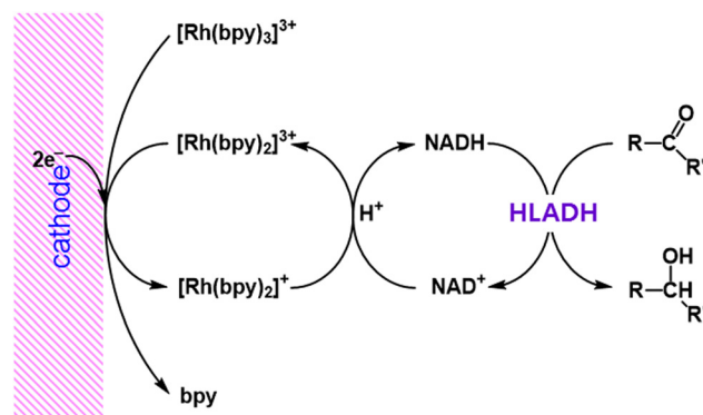
Scheme 3 Electrocatalytic production of NADH from \text{NAD}^+ using [\text{Rh}(\text{bpy})_2]^+ . 44
