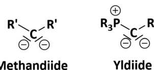
Fig. 1 ChemDraw showing methandiide versus yldiide ligands.
