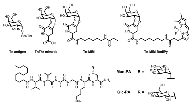
Fig. 1 Structure of the native Tn antigen, TnThr mimetic, alkyl derivative of the TnThr mimetic ( Tn-MIM ), and fluorescent TnThr mimetic ( Tn-MIM Bodipy ) and chemical structure of self-assembling peptide amphiphile molecules (Man-PA and Glc-PA).
