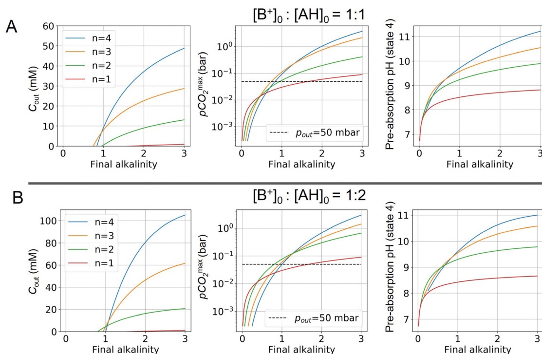
Fig. 4 ABCS process output. C_{\text{out}} (left), p_{\text{CO}_2}^{\text{max}} (middle), and \text{pH}_4 (right) are plotted as functions of final alkalinity. (A) [B^+]_0 : [AH]_0 = 1:1 ; (B) [B^+]_0 : [AH]_0 = 1:2 . Each reaction order is modelled with the corresponding optimal initial concentration and pK_{a,n} , taken from Fig. 3. For all points, p_{\text{in}} = 0.3 mbar; p_{\text{out}} is chosen at 50 mbar and denoted with a black dashed line in the middle plots.
