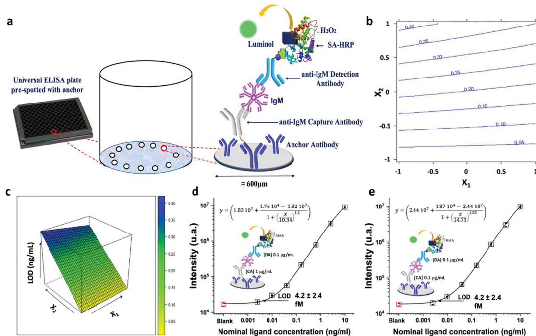
Fig. 4 (a) Scheme of the biosensor development; (b) isoresponse contour plot and (c) the response surface for LOD response. IgM calibration curve recorded using (d) 1 \mu\text{g mL}^{-1} and (e) 0.1 \mu\text{g mL}^{-1} of CA and DA anti-IgM antibodies respectively. Adapted and reproduced with permission from ref. 35. Copyright 2022, Wiley-VCH under Creative Commons Attribution 4.0 License (CC BY 4.0).
