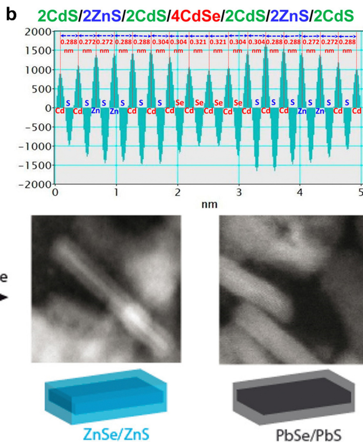
Fig. 11 (a) HAADF-STEM image of 2CdS/2ZnS/2CdS/4CdSe/2CdS/2ZnS/2CdS formed by c-ALD using Li 2 S/Li 2 Se and anhydrous Cd(HCOO) 2 /Zn(OAc) 2 powders as the sources of chalcogen and metal precursors, respectively; (b) the interplanar distances for this structure shown in (a); (c) schematic representation of the cation exchange of CdSe/CdS core/shell NPLs to ZnSe/ZnS and PbSe/PbS NPLs with corresponding HAADF-STEM images. Panels (a) and (b) are adapted with permission from The American Chemical Society. 240 Panel (c) is adapted with permission from The American Chemical Society. 254
