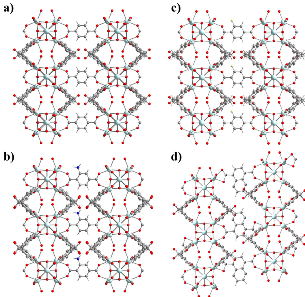
Fig. 3 Representations of the structures of (a) UCY-17(Tb)/BDC (b) UCY-17(Tb)/ABDC , and (c) UCY-17(Tb)/FBDC along the a axis and (d) UCY-17(Tb)/NDC along the b axis. Colour code: Tb, light blue; F, light yellow; O, red; N, blue; C, grey; and H, white.
