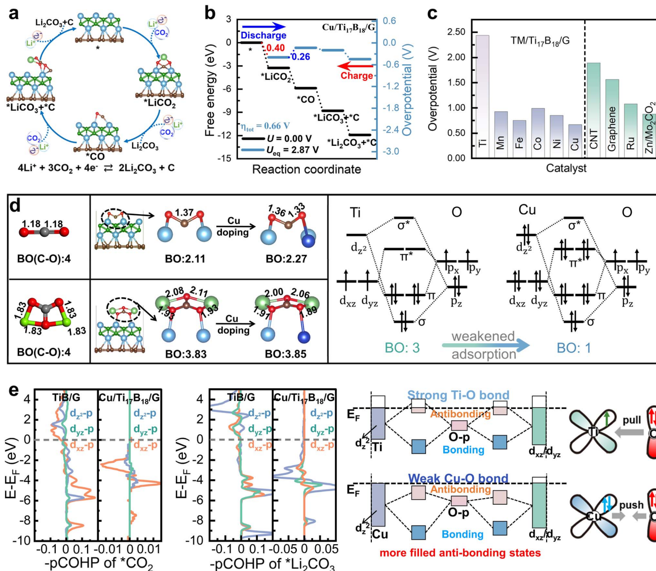
Fig. 3 (a) Continuous four-electron transfer pathway. (b) Free energy diagrams for \text{Cu}/\text{Ti}_{17}\text{B}_{18}/\text{G} , where blue and red numbers represent \text{CO}_2\text{RR} overpotential ( \eta_{\text{CO}_2\text{RR}} ) during discharge and \text{CO}_2\text{ER} overpotential ( \eta_{\text{CO}_2\text{ER}} ) during charge, respectively, and \eta_{\text{tot}} represents the total overpotential. (c) Comparison of total overpotential with available references. (d) Cu as a dopant reducing bond order (BO) in \text{CO}_2 and \text{Li}_2\text{CO}_3 adsorbates. (e) Evolutions of bonding and antibonding states in p-d orbital interactions, where the spin-up and spin-down channels are identical in the projected crystal orbital Hamiltonian population (pCOHP) due to the zero magnetic moment of the system.
