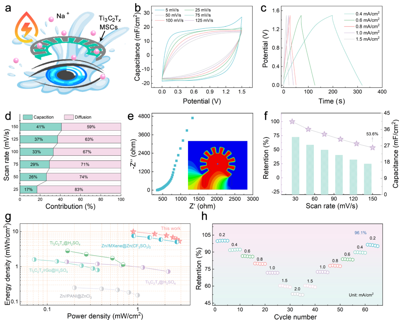
Fig. 3 (a) Schematic of the Ti 3 C 2 T x -MSCs. (b) CV curves at different scan rates. (c) GCD curves at different current densities. (d) Capacitive and diffusion contribution ratio of Ti 3 C 2 T x -MSCs at different scan rates. (e) EIS plots and simulated energy distribution of Ti 3 C 2 T x -MSCs. (f) Variation of areal capacitance and capacitance retention with various scan rates. (g) Ragone plot of areal energy density vs. power density for Ti 3 C 2 T x -MSCs in comparison with the reported MSCs. (h) The rate properties of the Ti 3 C 2 T x -MSCs at different current densities.
