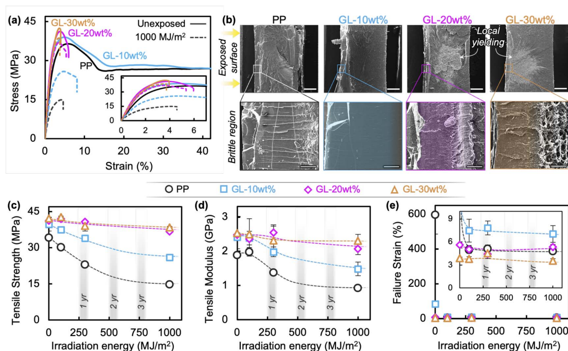
Fig. 4 (a) Stress–strain curves for specimens before and after irradiation (1000 MJ m -2 ). (b) SEM images of fracture surfaces of specimens after 1000 MJ m -2 of irradiation, showing a transition from brittle surface crack growth to post-yield fracture behavior (scale bars are 500 μm for top, 50 μm for bottom). Summaries of (c) tensile strength, (d) elastic modulus, and (e) failure strain at different irradiation energies and their equivalent sunlight exposure times; lines are intended to guide the eyes.
