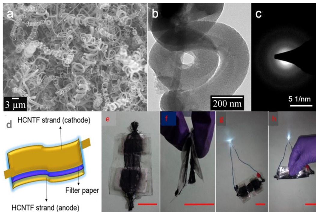
Fig. 28 (a) SEM; (b)TEM; and (c) SAED images of HCNTF having an HCNT density of 5.77 \text{ mg cm}^{-3} ; (d) pictorial representation of fabricated device; (e) series connection of two solid state flexible HCNTFs; (f) bending of module at 180^\circ ; (g) discharging of module by LED; and (h) discharging of module by a white LED with bending at 180^\circ . Reproduced with permission from ref. 63 Copyright (2016), Elsevier.
