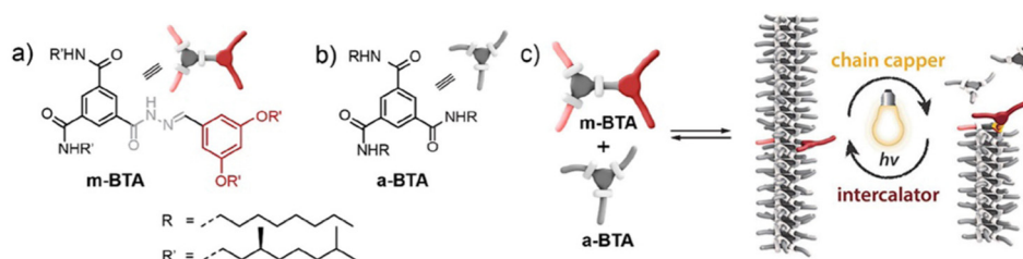
Fig. 30 Molecular structure of (a) mono acylhydrazone functionalized BTA (m-BTA), (b) achiral octyl BTA (a-BTA) monomers, and (c) copolymer formed by intercalation of chiral m-BTA into helical stacks of a-BTA. Light induced isomerisation of the acylhydrazone linkage in m-BTA converts it into a chain stopper, and shortens the length of the assembled nanofibers. Figure reproduced adapted from ref. 251 with permission of the American Chemical Society, © 2020.
