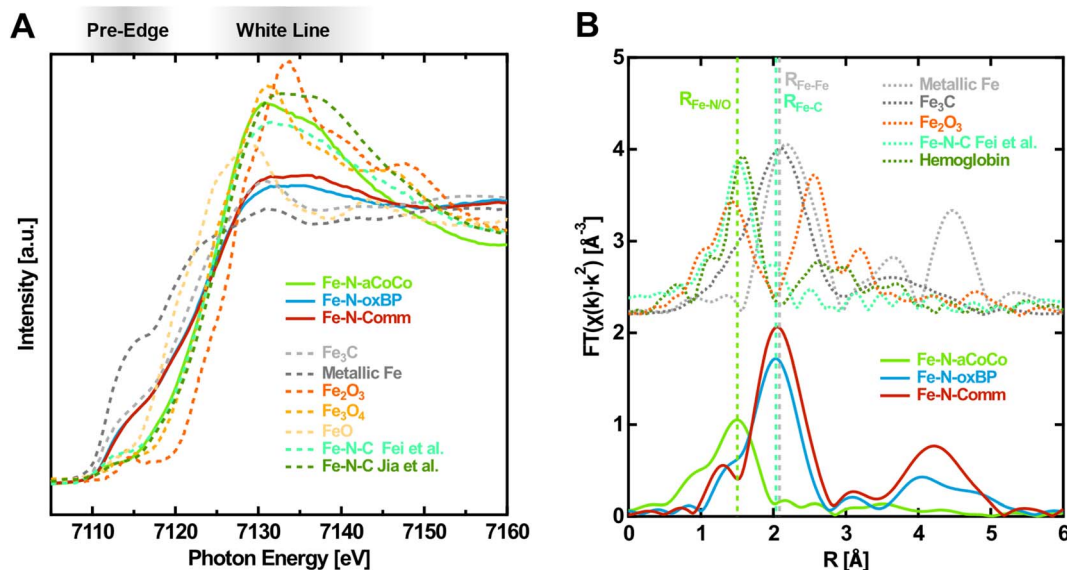
Fig. 1 Fingerprinting at the Fe K-edge of the Fe–N–C catalysts in the oxidized state (1.0 V vs. RHE applied). (A) XANES-region of the Fe K-edge with references of iron carbide 29 ( Fe_3C ), metallic iron, iron oxides 30 ( Fe_2O_3 , Fe_3O_4 , and FeO ) and different Fe–N–C materials (from Fei et al. 28 and Jia et al. 27 ). (B) Fourier transform of the EXAFS-region with references of iron carbide 29 ( Fe_3C ), metallic iron, iron oxide 23 ( Fe_2O_3 ) and an exemplary Fe–N–C material from Fei et al. 28 and glycated hemoglobin. 31
