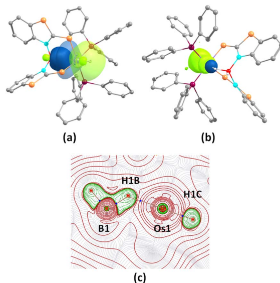
Fig. 6 (a) Donor–acceptor interaction between \sigma(\text{B–H}) and the Os center in 4a ; (b) Os–H bonding interaction in 4a (isovalue 0.004 [ e \text{ bohr}^{-3} ] 1/2 ); (c) contour-line diagram of the Laplacian of the electron density along Os–H–B planes in 4a .
