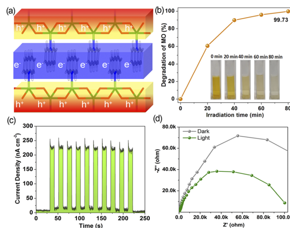
Fig. 6 (a) A schematic diagram of the arrangement of electrons and hole transport channels in 1 . (b) Percentage photocatalytic degradation of the methyl orange dye (20 mg L⁻¹) in the presence of powdered 1 (10 mg) in a neutral aqueous solution. Insets show the photos of MO aqueous solution after different illumination times. (c) Transient photocurrent measurements of 1 under repeated on/off cycles of illumination at 0 V vs. Ag/AgCl. (d) Electrochemical impedance spectroscopy Nyquist plots of the powder of 1 coated on ITO under dark and illumination conditions without additional bias potential.
