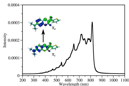
Fig. 5 Vibrationally resolved triplet–triplet spectrum of DETC for its T_1 \rightarrow T_4 transition employing T_1 as starting geometry. Visualization of the electronic density difference in T_1 and T_4 excited states compared to the electronic structure of DETC in the ground state is reported in the inset. Electron donating regions, i.e. holes, and electron accepting, i.e. electrons, are marked in blue and green, respectively. An isovalue of 0.002 a.u. was used for visualization.
