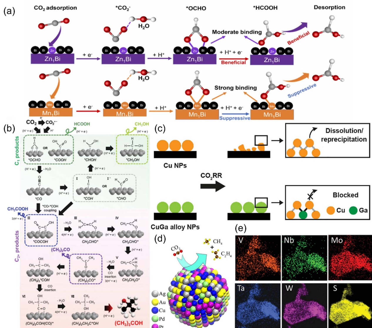
Fig. 21 (a) A proposed reaction mechanism for \text{CO}_2\text{R} to formate on SAA- \text{Zn}_1\text{Bi} and SAA- \text{Mn}_1\text{Bi} . (b) A probable mechanism for \text{CO}_2\text{R} to (\text{CH}_3)_3\text{COH} . (c) Illustration of the \text{CO}_2\text{RR} stabilization mechanism on CuGa alloy NPs. (d) Schematic of the catalysis reaction on AuAgPtPdCu. (e) EDS maps of (\text{MoWVNBa})\text{S}_2 . (a) Reproduced with permission. 233 Copyright 2023, Elsevier Ltd. (b) Reproduced with permission. 236 Copyright 2023, Wiley-VCH GmbH. (c) Reproduced with permission. 237 Copyright 2023, American Chemical Society. (d) Reproduced with permission. 240 Copyright 2020, American Chemical Society. (e) Reproduced with permission. 241 Copyright 2021, Wiley-VCH GmbH.
